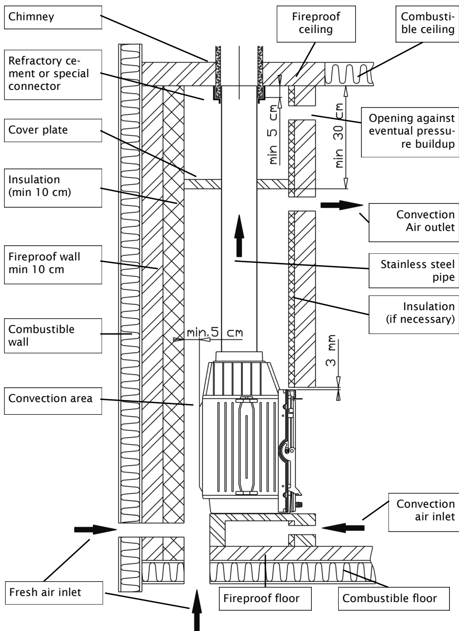
Example of fireplace installation within combustible material
